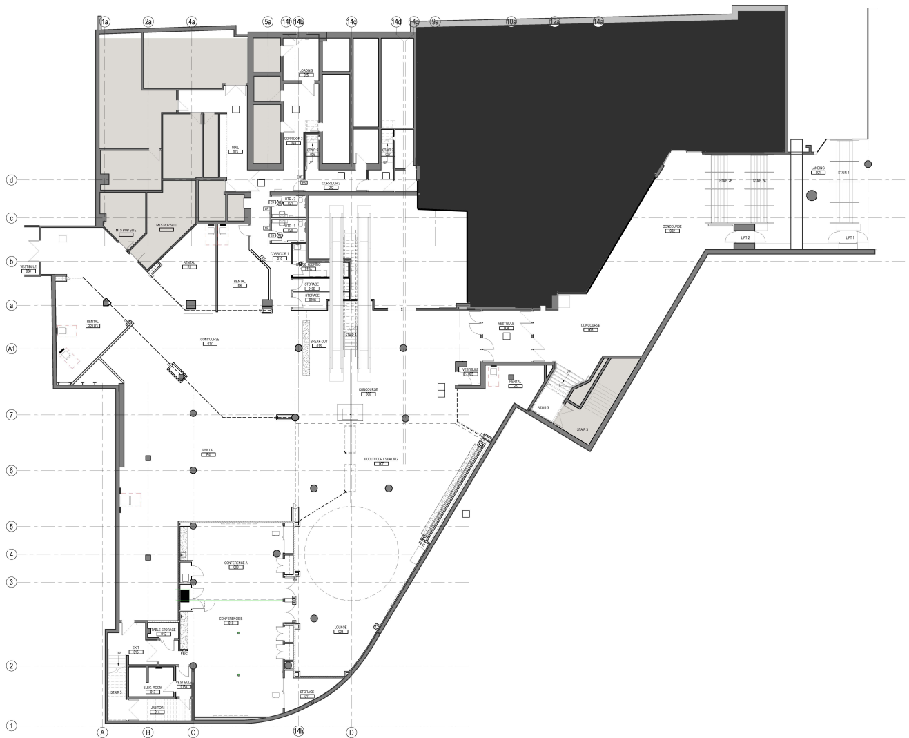
1 CONCOURSE - PLAN 1/8\" = 1'-0\"
